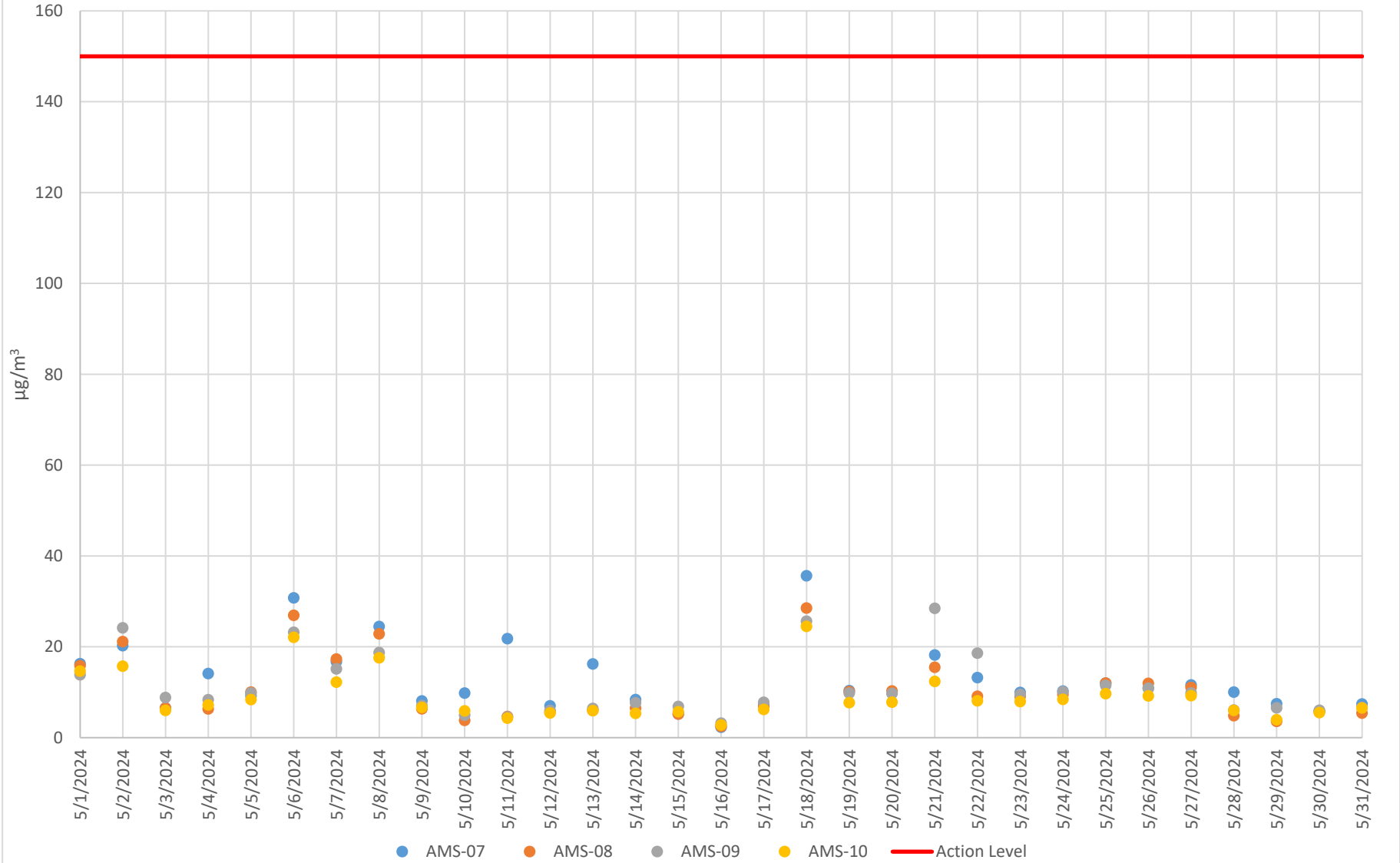
Figure 2.b - Dust Concentration 24-Hour Averages Innovation Campus May 1, 2024 – May 31, 2024 The Bellwether District
