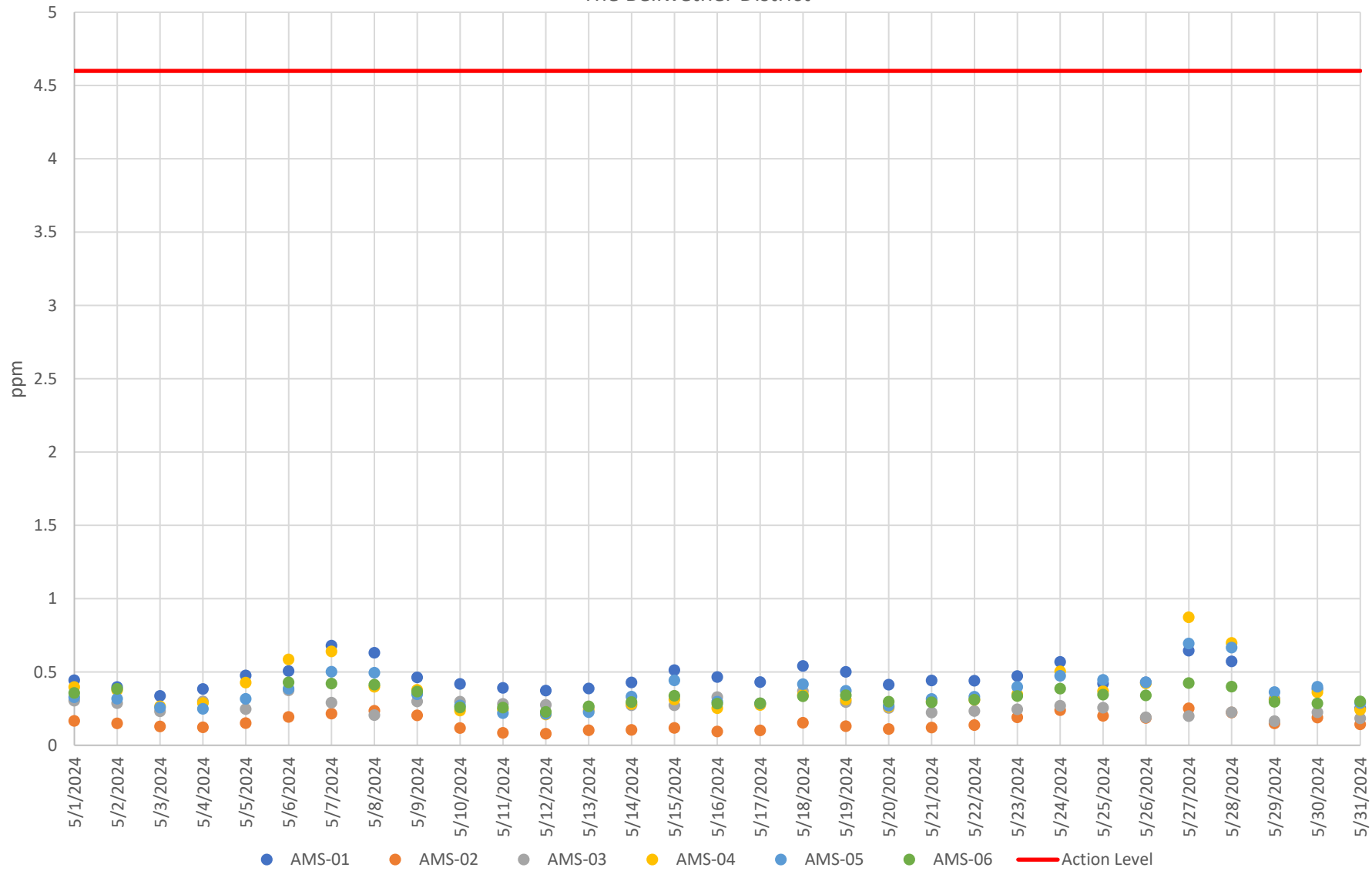
Figure 3.a - VOC Concentration 8-Hour Averages Industrial Campus May 1, 2024 – May 31, 2024 The Bellwether District
