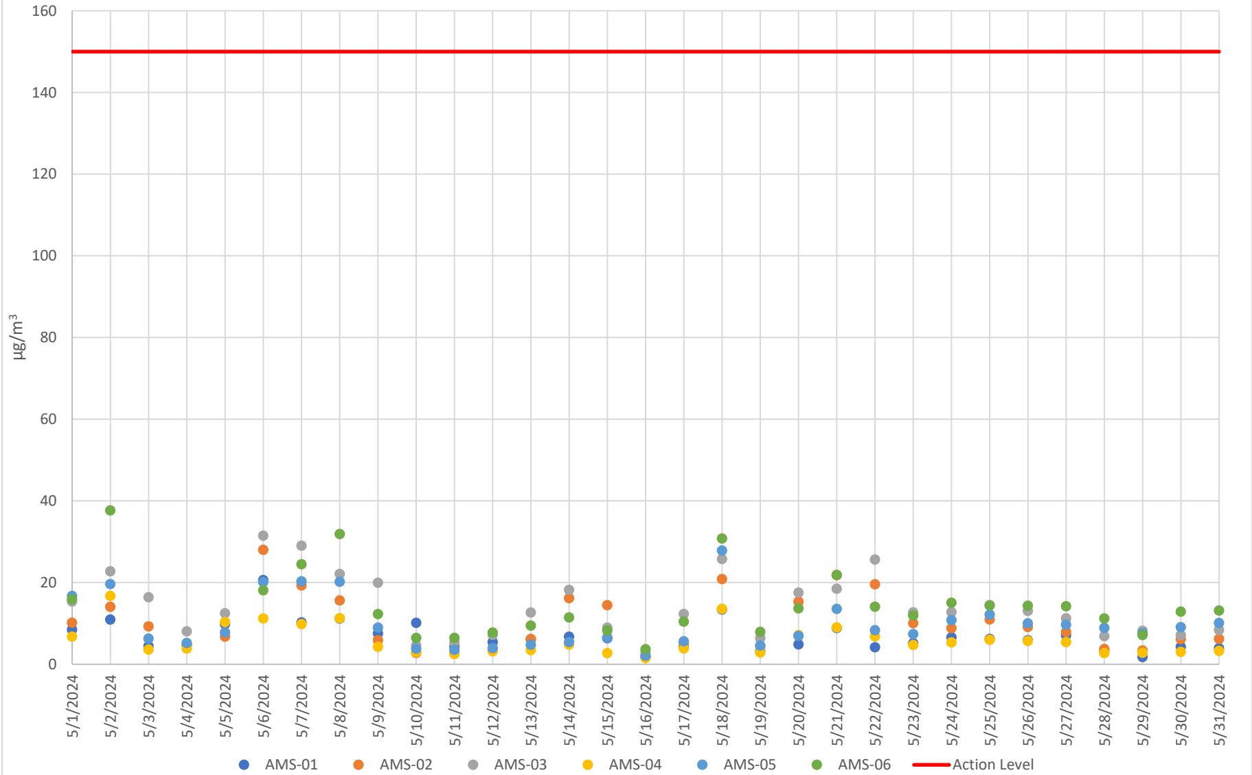
Figure 2.a - Dust Concentration 24-Hour Averages Industrial Campus May 1, 2024 – May 31, 2024 The Bellwether District
