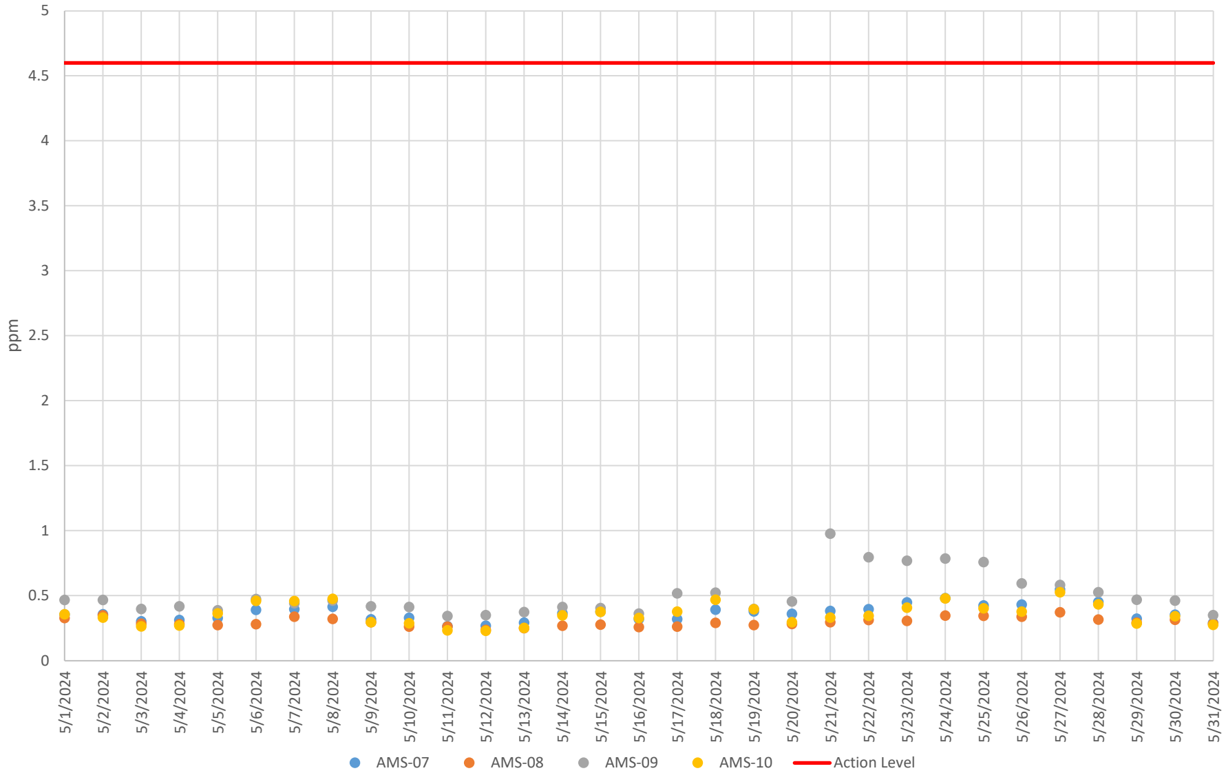
Figure 3.b - VOC Concentration 8-Hour Averages Innovation Campus May 1, 2024 – May 31, 2024 The Bellwether District
